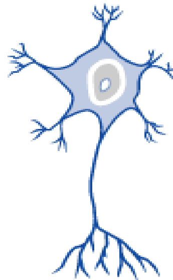
Multipolar (Motoneuron)
